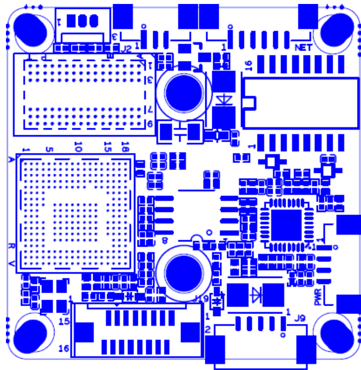
P5 power
