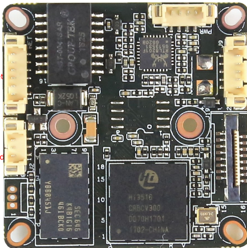
P5 power
